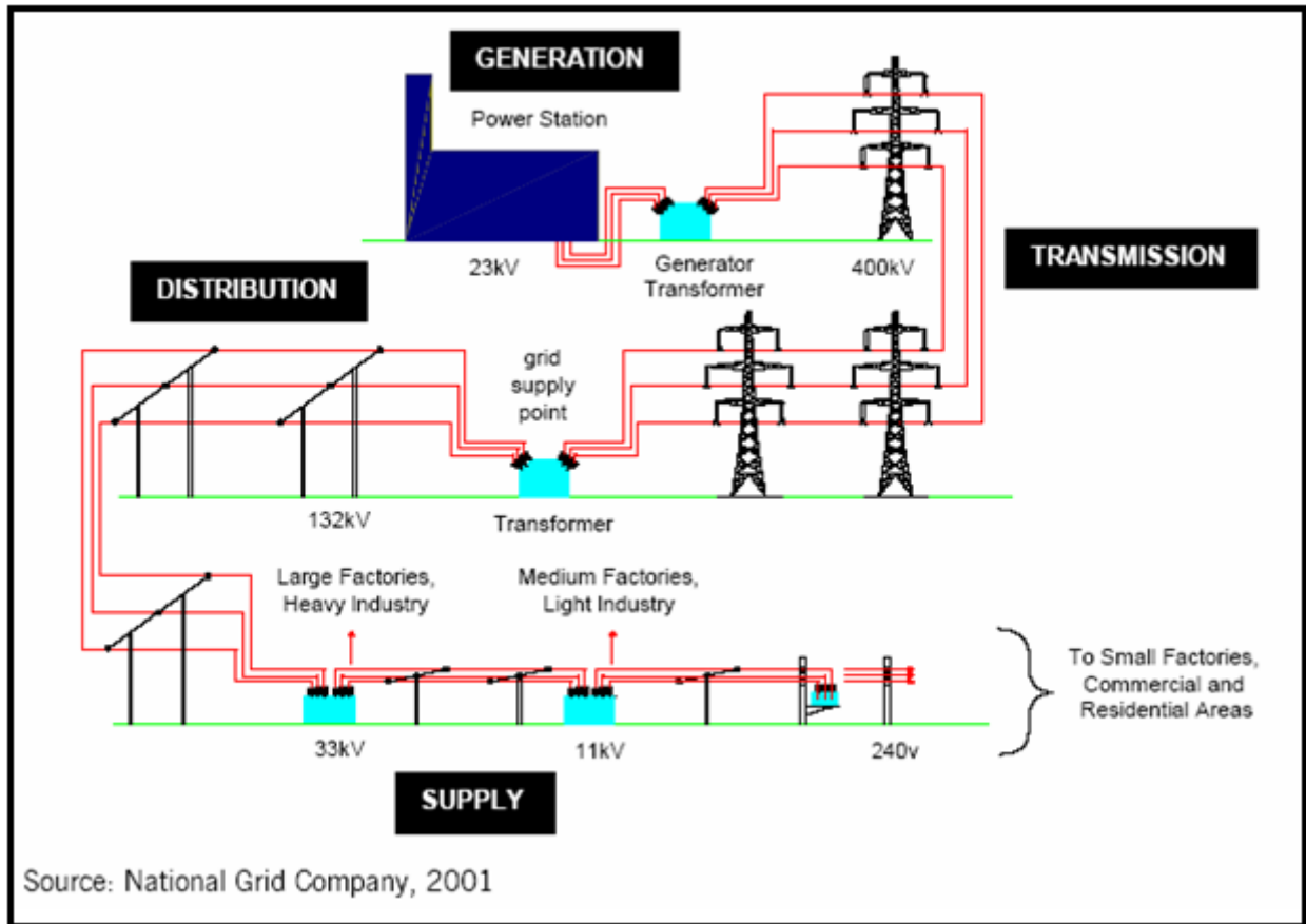
Fig.1. Line diagram of power system
