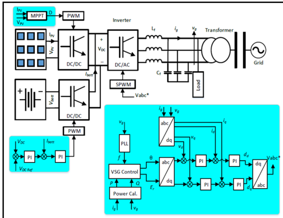
Fig.3. Complete block diagram of proposed approach
