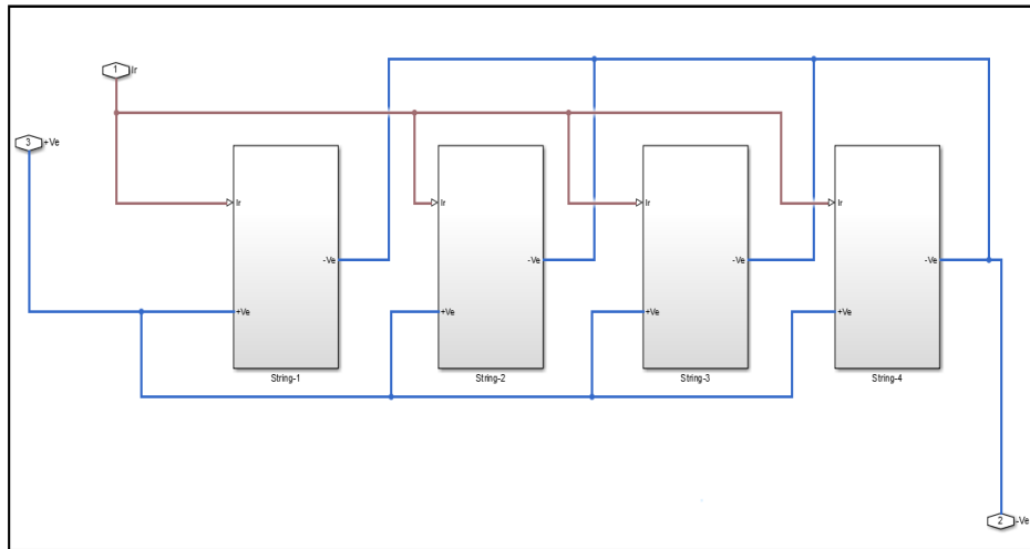
Fig.8. MATLAB simulink model of parallel connected all solar strings subsystem in 5 KW solar array systems
