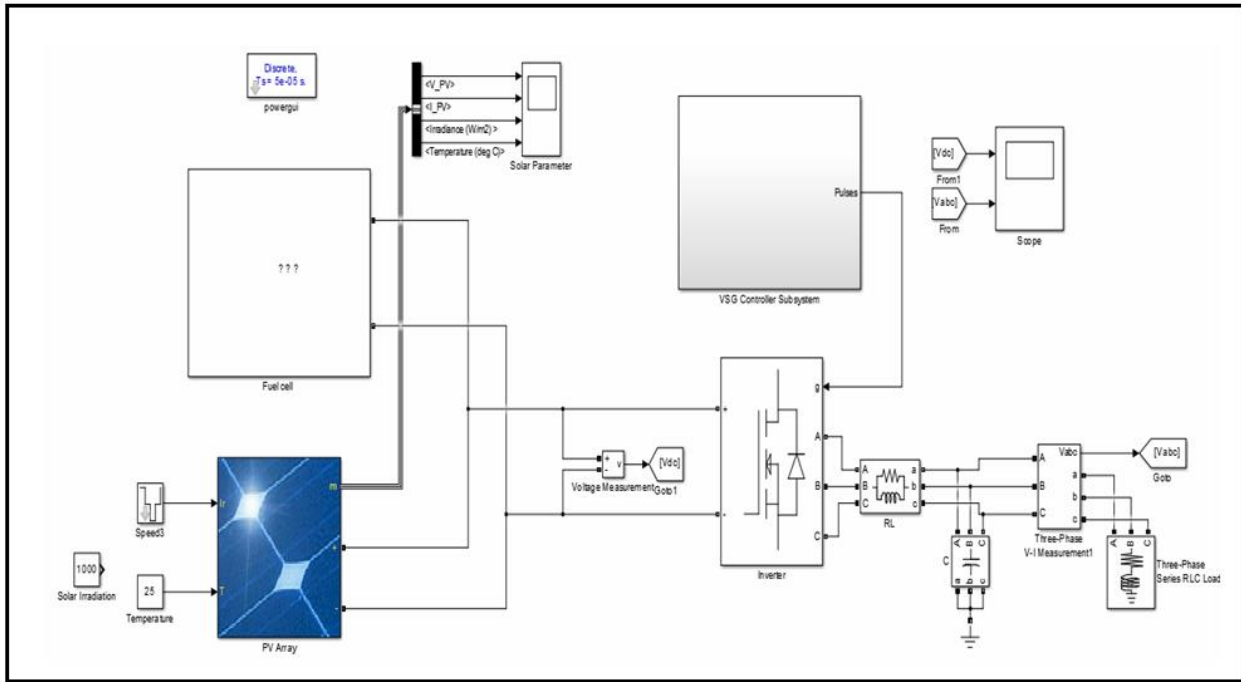
Fig.15. Compete matlab simulation model
