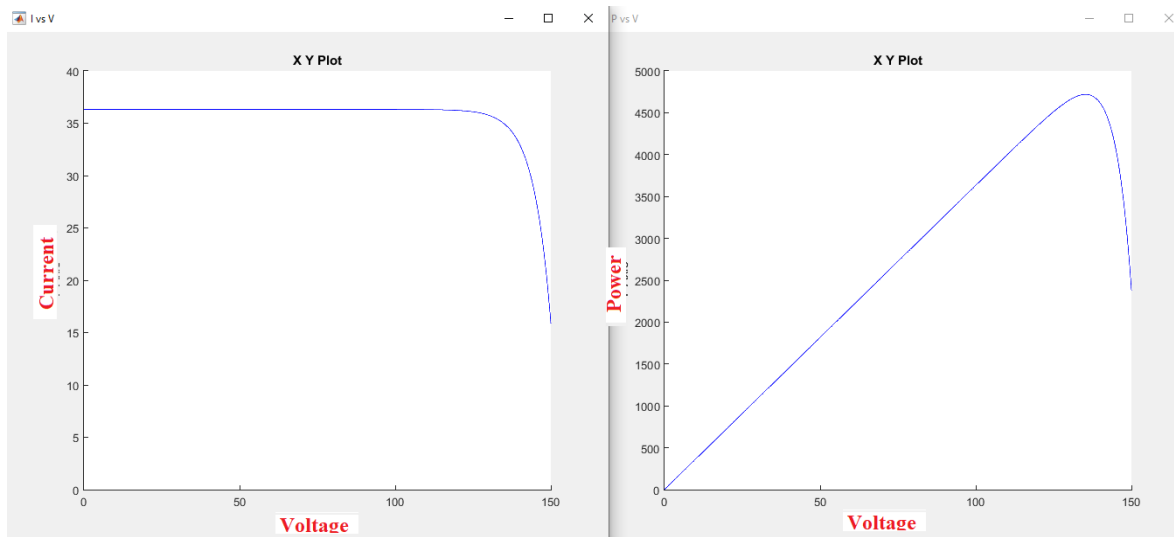
Fig.9. VI and PV characteristics of 5 KW solar PV array at 1000 \text{ W/m}^2 irradiation using MATLAB simulink modeling
