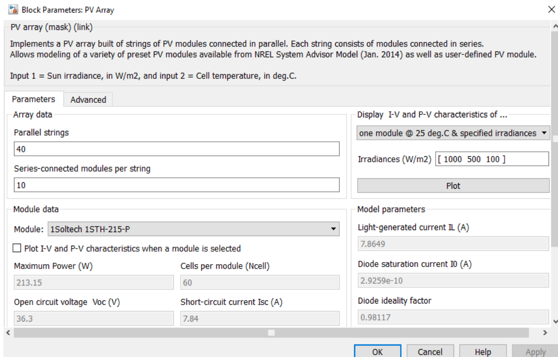
Fig.10. MATLAB simulink specification window of model of solar pv array system
