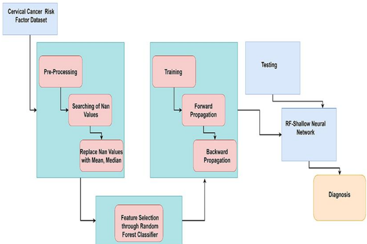
Fig 2. Machine Learning Assisted Cervical Cancer Detection
